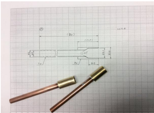
Dual mode Horn
